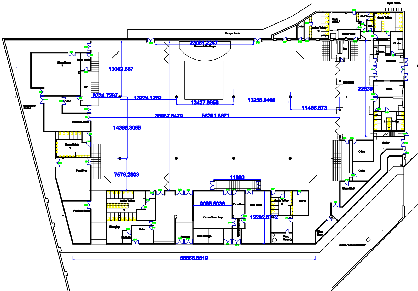
GROUND FLOOR LAYOUT PLAN
